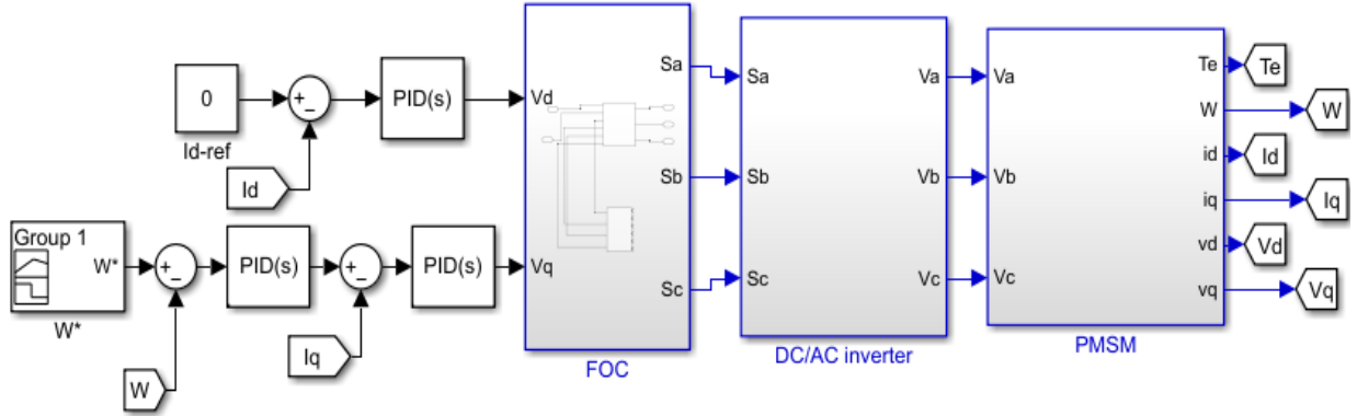
Fig. 1. Matlab block diagram of FOC for PMSM.
