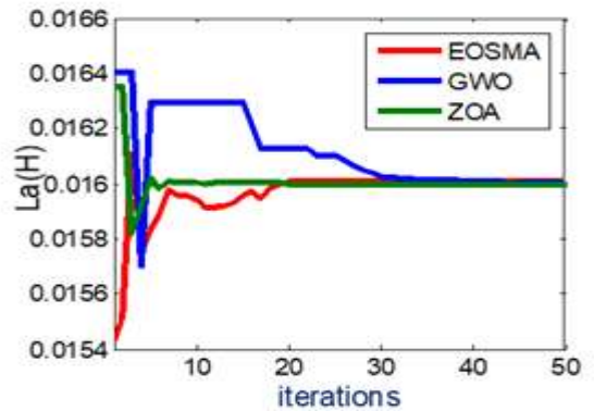
Fig. 3. Armature Inductance
