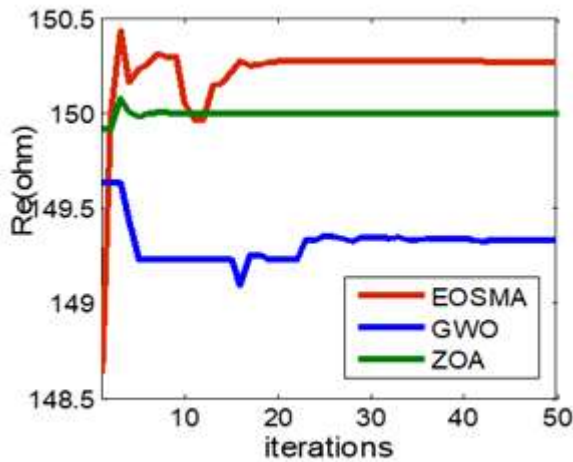
Fig. 6. Field Resistant
