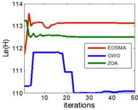
Fig. 5. Field Inductance.
