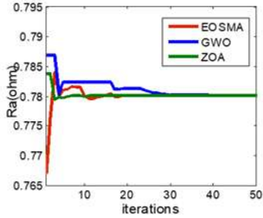
Fig. 4. Armature Resistance.
