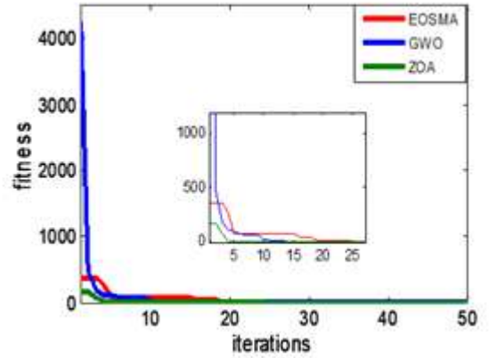
Fig. 2. Objective function.
